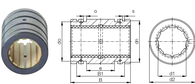
Closed, anodised aluminium adapters - 01 version (standard)
