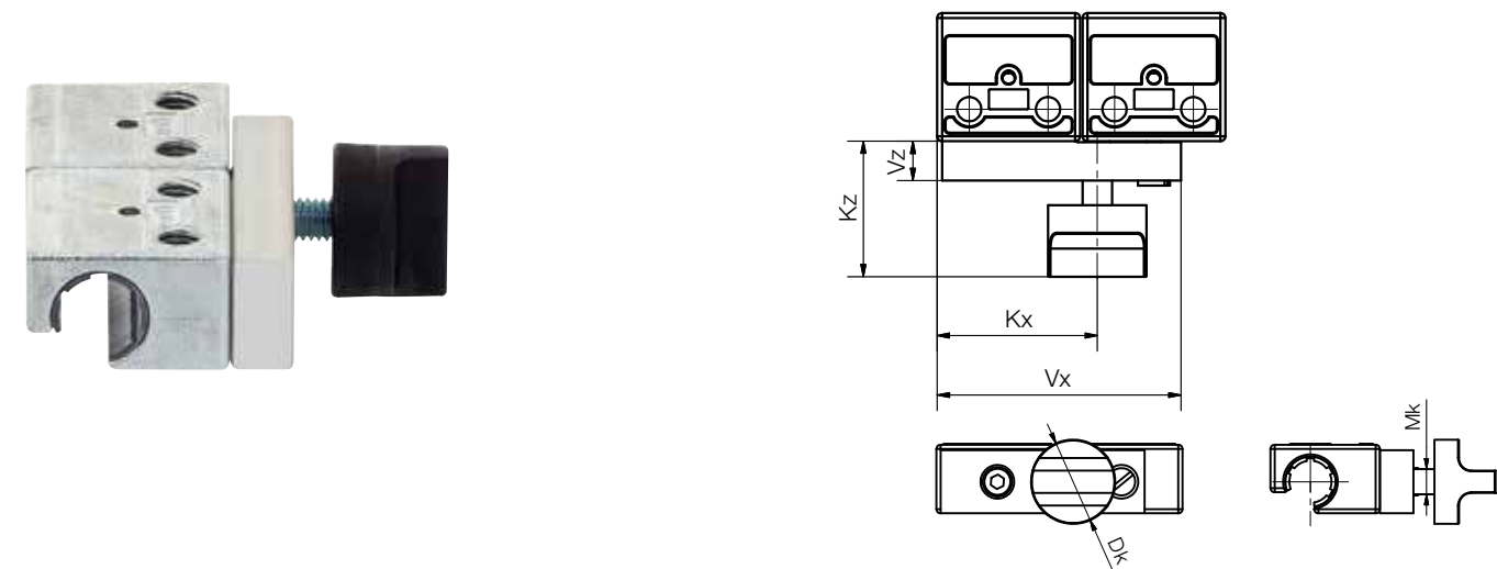
Technical data and dimensions [mm]
