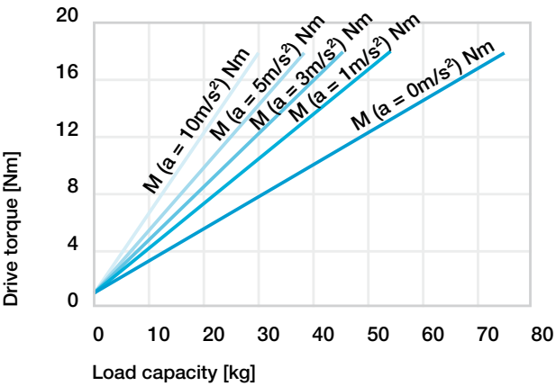
Diagram 16: Required drive torque 140) ; vertical orientation - ZLW-20120, version standard 02
