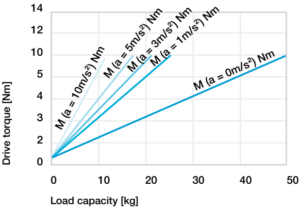
Diagram 14: Required drive torque 140) ; vertical orientation - ZLW-1660, standard 02 version
