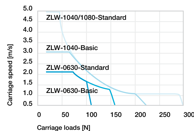
Diagram 11: Maximum load compared: ZLW-0630 and ZLW-1040/1080, 100% ED (duty cycle). The graph accounts for the sum of all forces active on the carriage.
