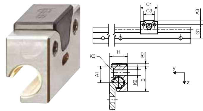
WJRM-01 with single roller
