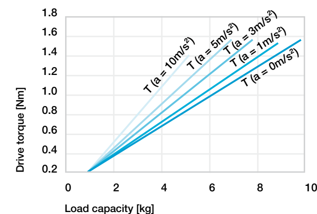
Diagram 08: Required drive torque 139) ; vertical orientation - ZLW-1040, basic 02 version
