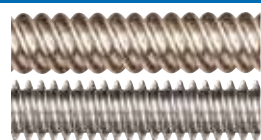
dryspin® lead screws with standard pitches
