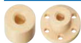
Cylindrical lead screw nuts, Injection-moulded lead screw nuts with flange lead screw nuts with metric machined thread
