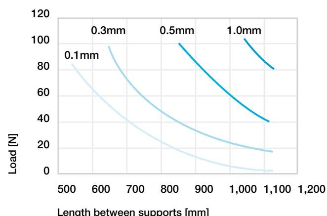
Diagram 06: Sag between unsupported end blocks ZLW-0630, basic 02 and standard 02 version. Sag permissible up to 2mm maximum.
