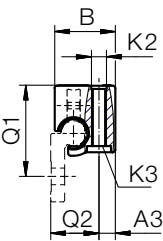
WJRM-31 Installation position 01
