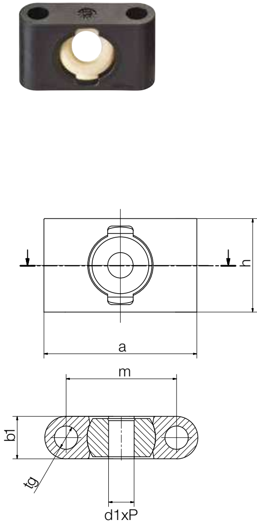
Dimensions [mm] - trapezoidal thread
