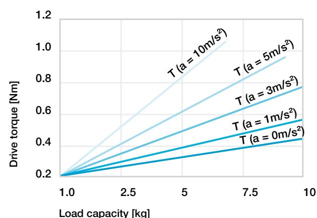
Diagram 03: Required drive torque 138) ; horizontal orientation - ZLW-0630, version standard 02
