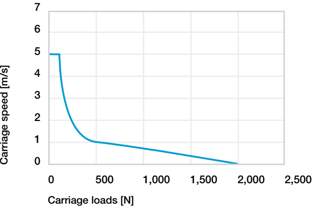
Diagram 15: Maximal load, horizontal installation; the graph accounts for the sum of all forces active on the carriage.
