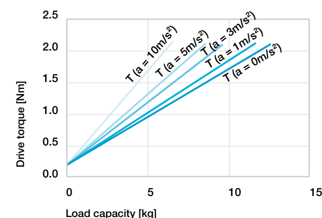
Diagram 10: Required drive torque 139) ; vertical orientation - ZLW-1040/1080, version standard 02
