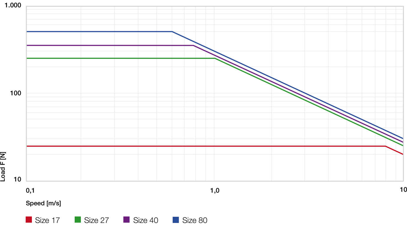
Diagram 01: F v diagram, maximum permissible dynamic load
