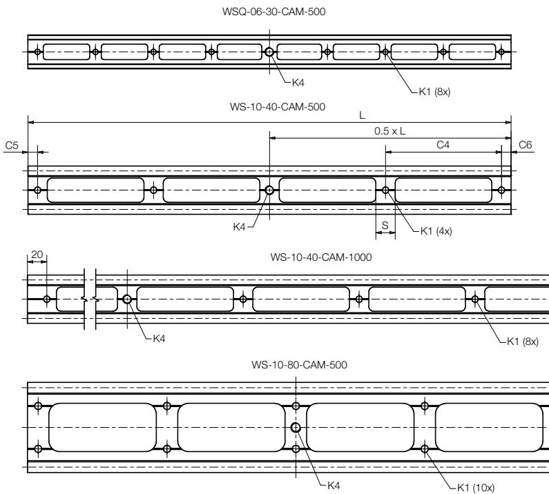
drylin® W guide rails - dimensions [mm]
