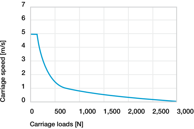
Diagram 18: Maximal load, horizontal installation; the graph accounts for the sum of all forces active on the carriage.
