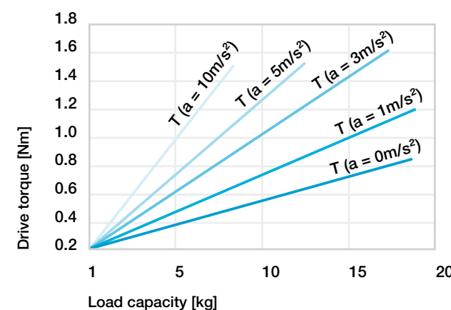
Diagram 07: Required drive torque 139) ; horizontal orientation - ZLW-1040, version basic 02
