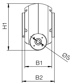
Technical data and dimensions [mm] - with turntable on both sides
