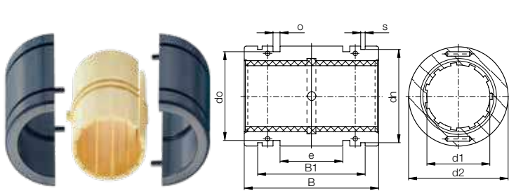
Split aluminium adapters - 01 version (standard)
